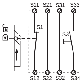
Fig. 5: Control de puerta protectora monocal, rearme supervisado/Controllo monocal riparo mobile, start controllato/Eenkanalige hekbewaking, bewaakte start
